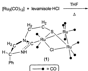
Scheme 1. Synthesis of compound 1
